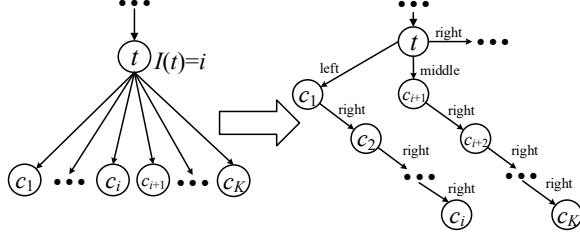
Figure 4: The canonicalization for node t .
