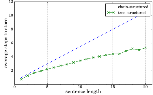
Figure 6: Average number of steps need to be stored for hidden states in both structures.
